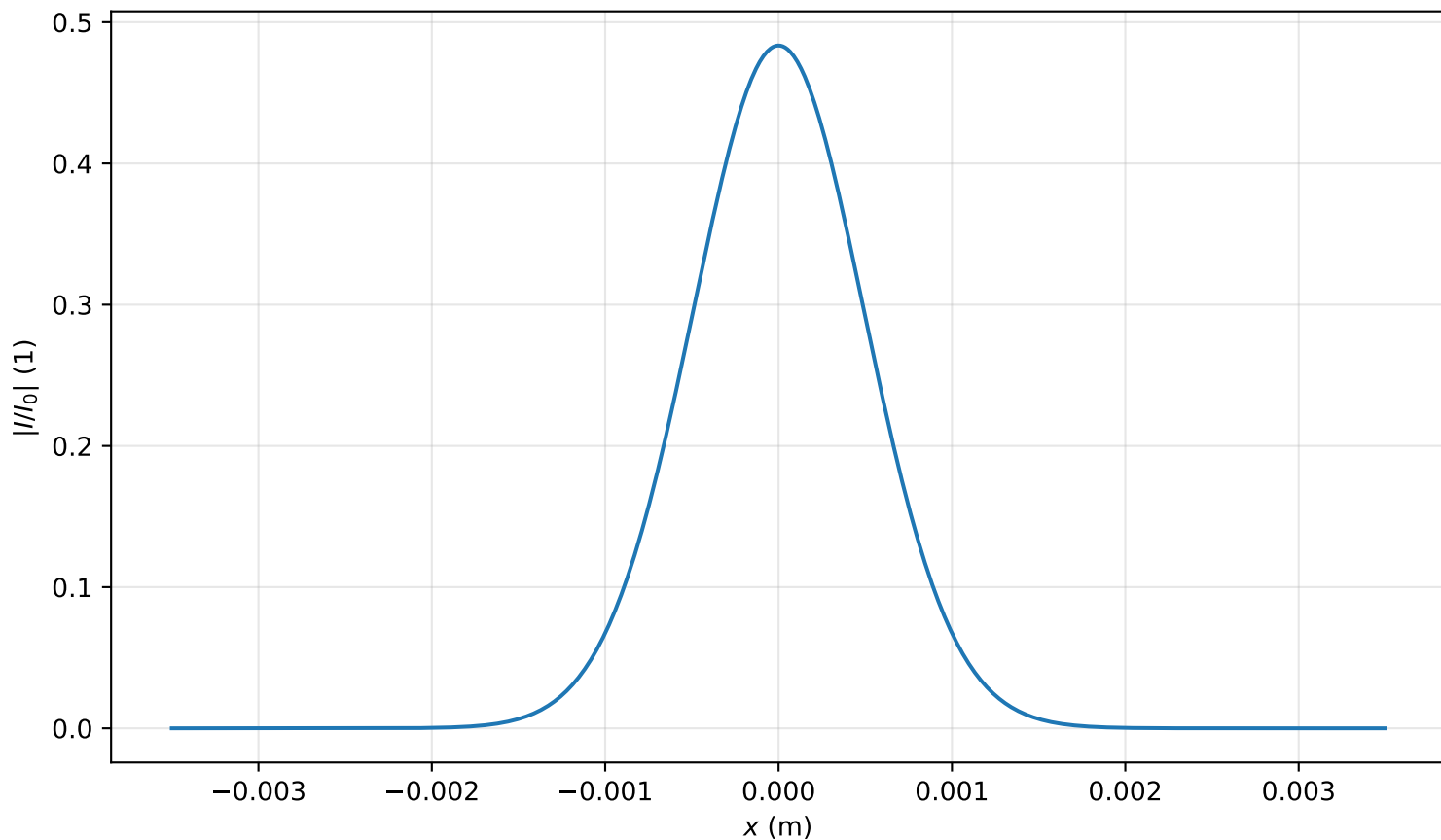
Intensity profile I(x, y = 0, z = 2.229m)/I_0 , P_{in}=0.1P_{cr} , artificial time
